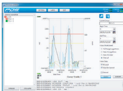
PDSSimply Local Monitoring Mode
